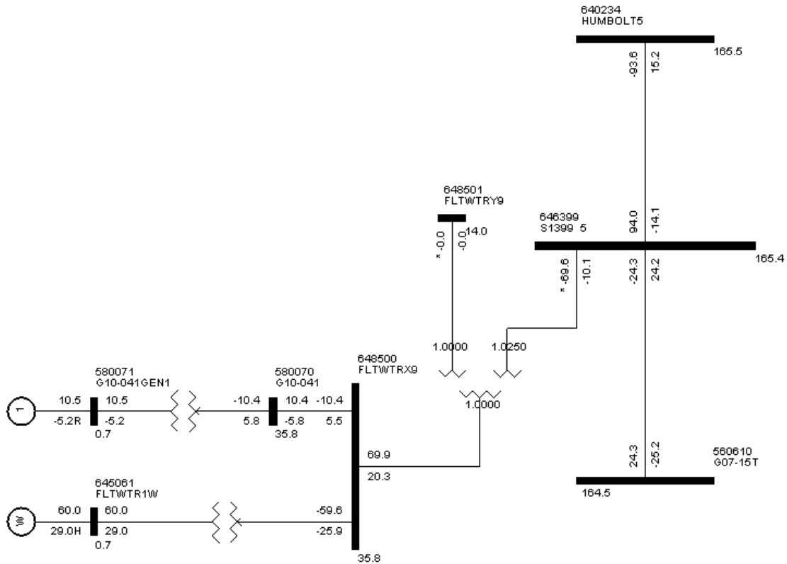
Figure 2-3: GEN-2010-041 Conceptual One-Line Diagram
